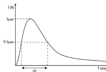
Example of a typical inrush current graph
