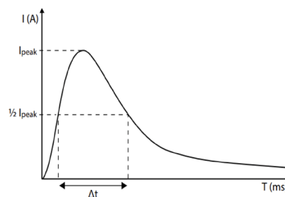
Example of a typical inrush current graph
